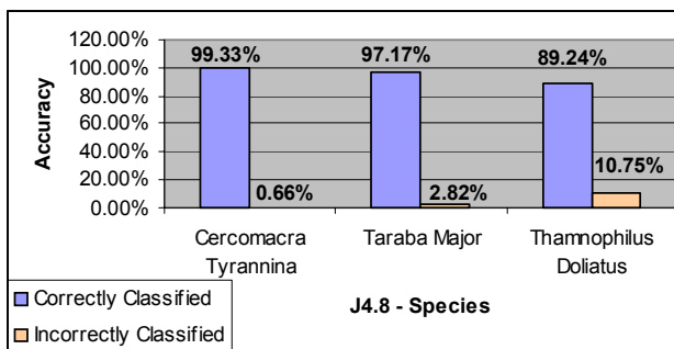
Figure 3. J4.8 accuracy percentages graph
