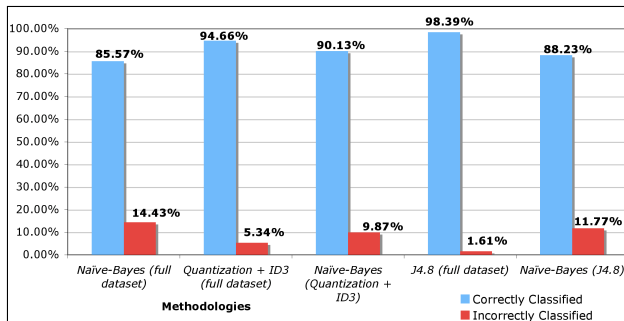
Figure 2. Data Mining accuracy percentages plot
